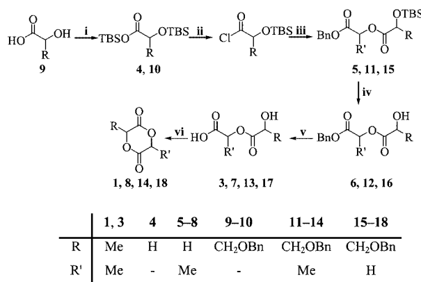
Scheme 4. i) 2.1 equiv. TBSCl, imidazole, DMF. ii) (\text{COCl})_2 , cat DMF, DCM. iii) benzyl ( S )-lactate/benzyl glycolate, pyridine, \text{Et}_2\text{O} . iv) TBAF/ \text{HOAc} , \text{EtOAc} . v) 1 equiv. w/w \text{Pd/C} , 1,4-cyclohexadiene, \text{EtOH} . vi) cyanuric chloride, acetone, \text{Et}_3\text{N}
